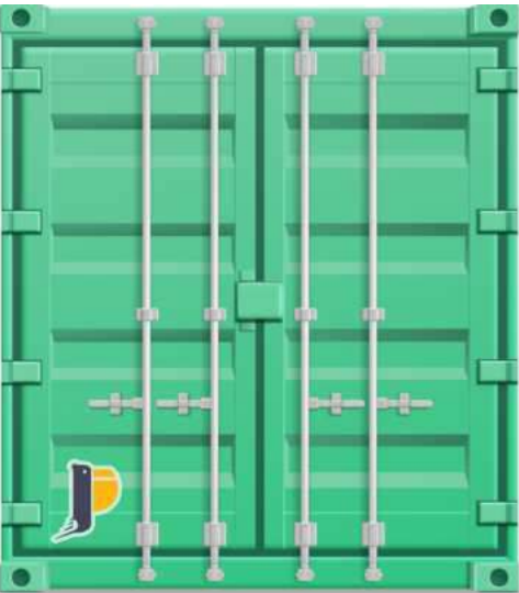
Container Read
